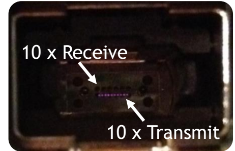
100GBASE-SR10 CXP
