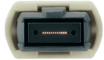
12-Fiber MPO Cable Connector
