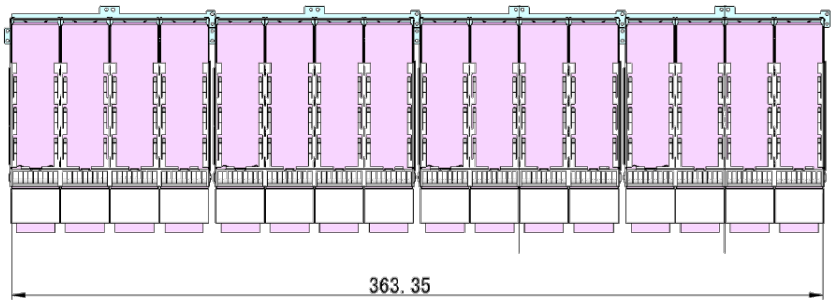
CFP4 16 Ports Per Card Front Panel Density
